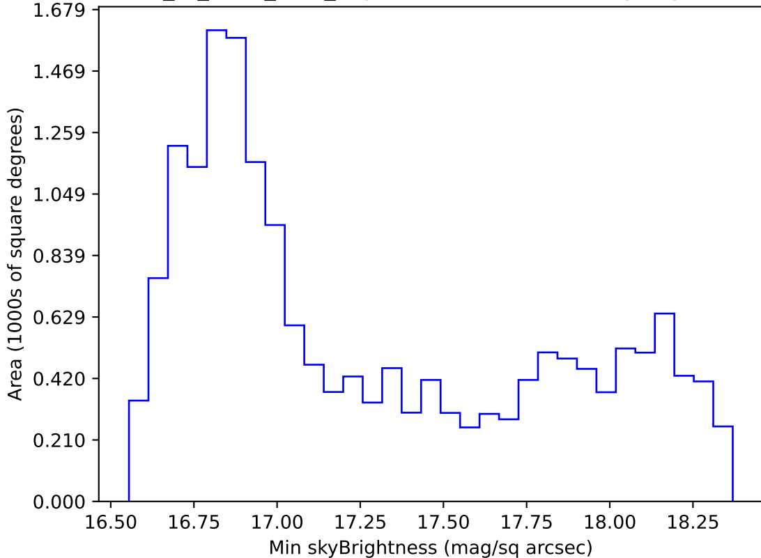
extra_ss_neo3_v3.4_10yrs WFD z band: Min skyBrightness
