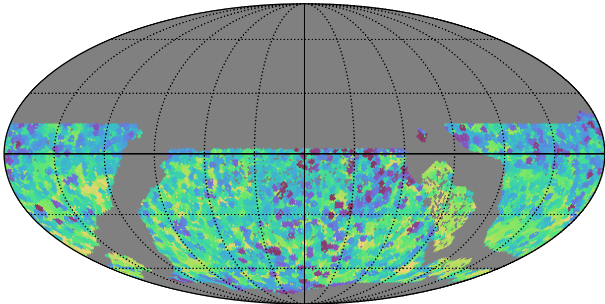
extra_ss_neo3_v3.4_10yrs WFD y band: Min skyBrightness
