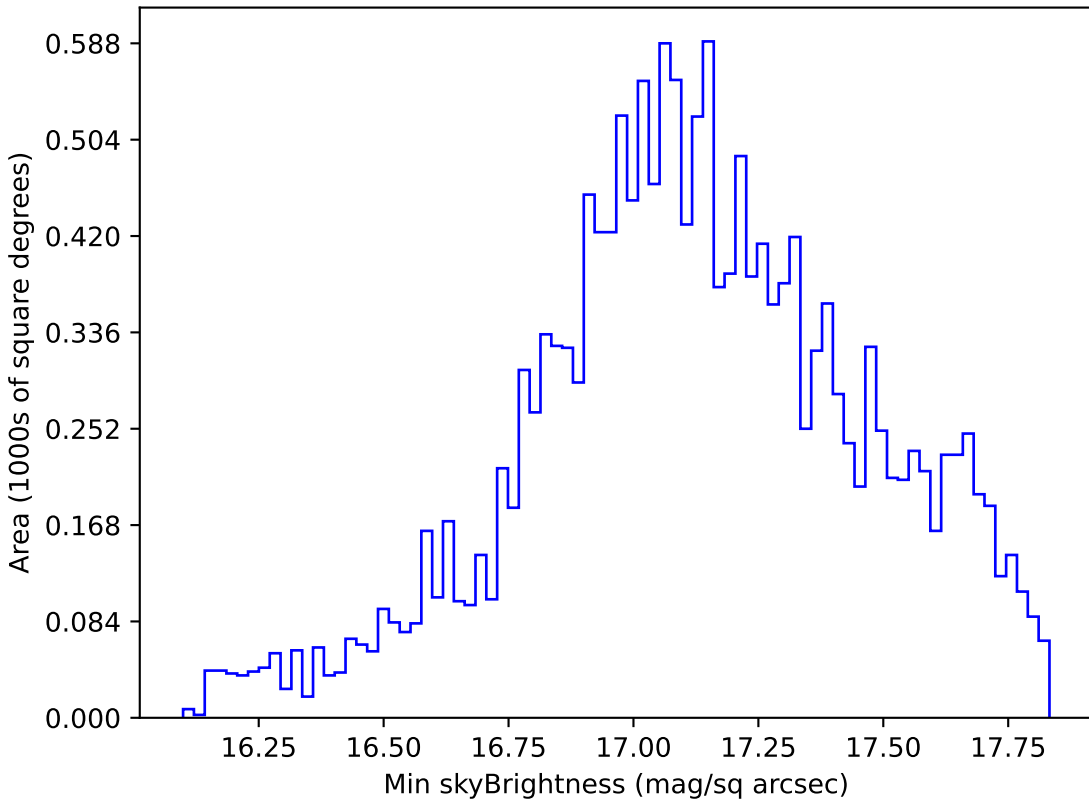
extra_ss_neo3_v3.4_10yrs WFD y band: Min skyBrightness
