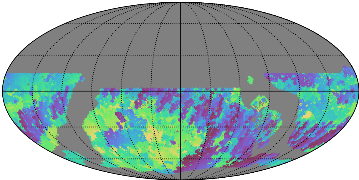
extra_ss_neo3_v3.4_10yrs WFD r band: Min skyBrightness
