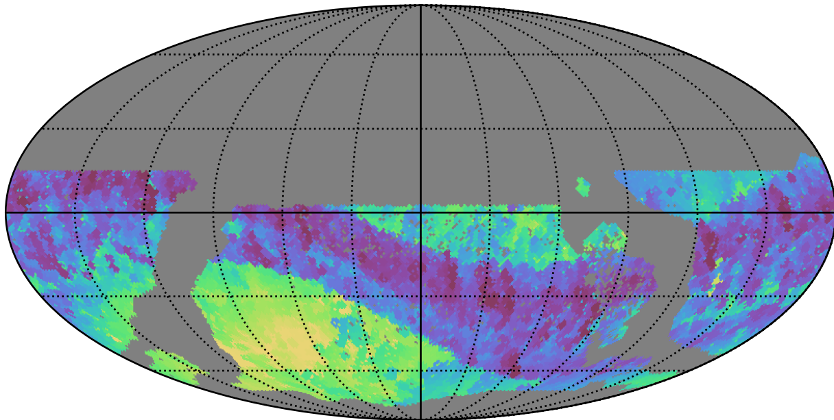
extra_ss_neo3_v3.4_10yrs WFD i band: Min skyBrightness
