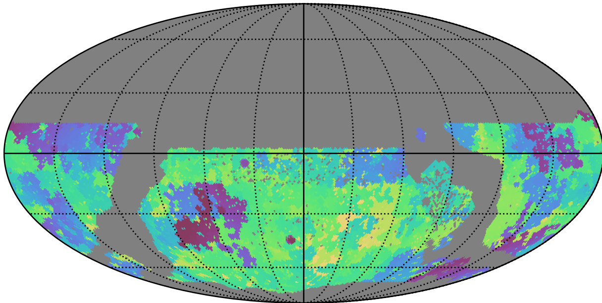
extra_ss_neo3_v3.4_10yrs WFD g band: Min skyBrightness
