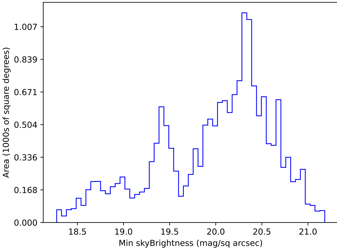
extra_ss_neo3_v3.4_10yrs WFD g band: Min skyBrightness
