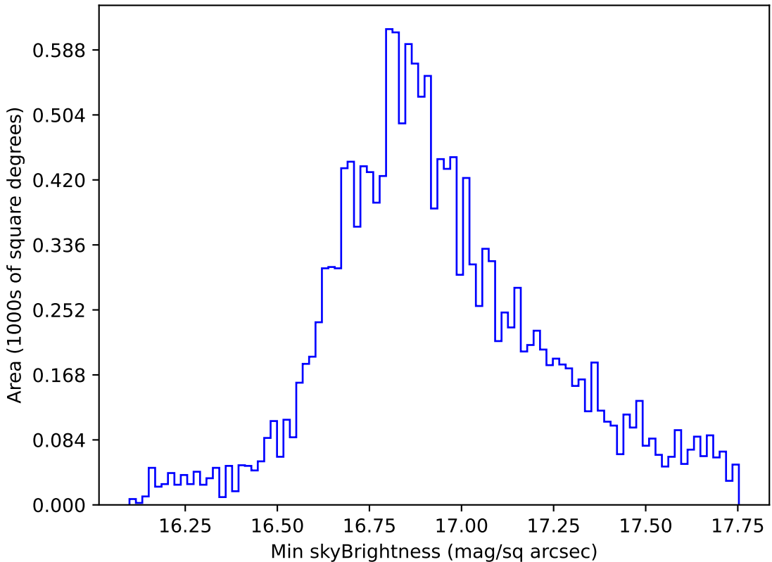
extra_ss_neo3_v3.4_10yrs WFD all bands: Min skyBrightness
