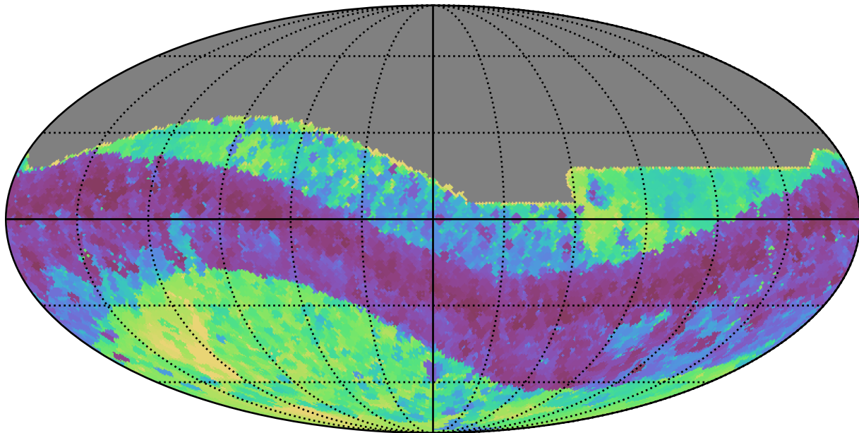
extra_ss_neo3_v3.4_10yrs All sky z band: Min skyBrightness
