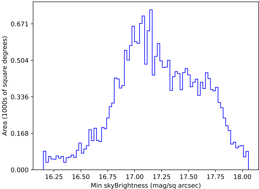
extra_ss_neo3_v3.4_10yrs All sky y band: Min skyBrightness
