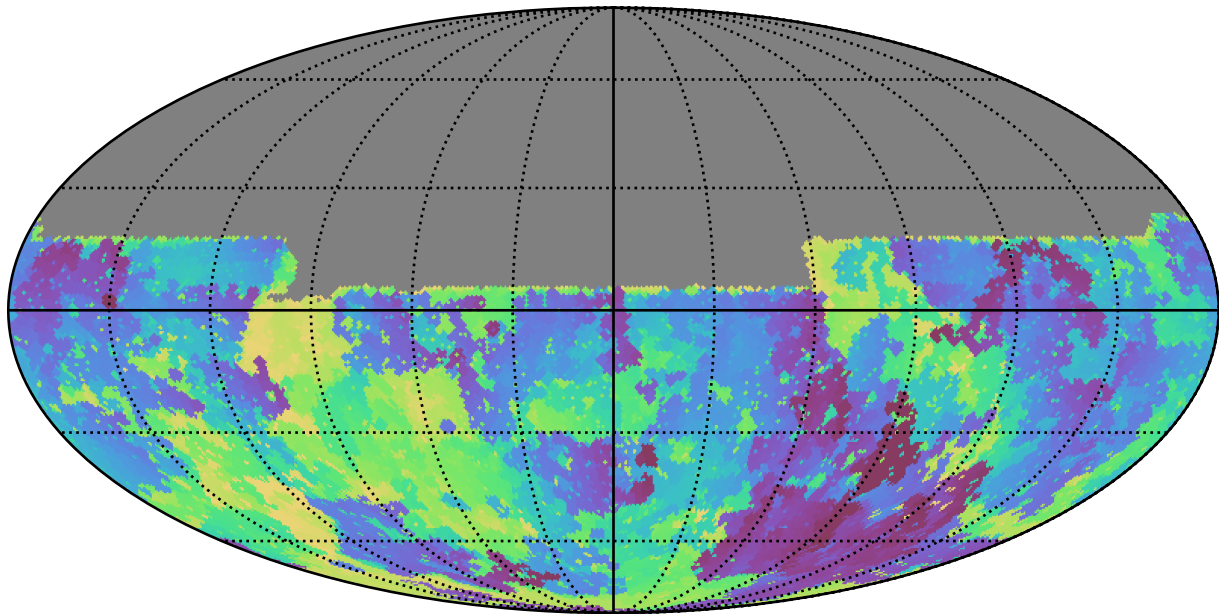
extra_ss_neo3_v3.4_10yrs All sky u band: Min skyBrightness
