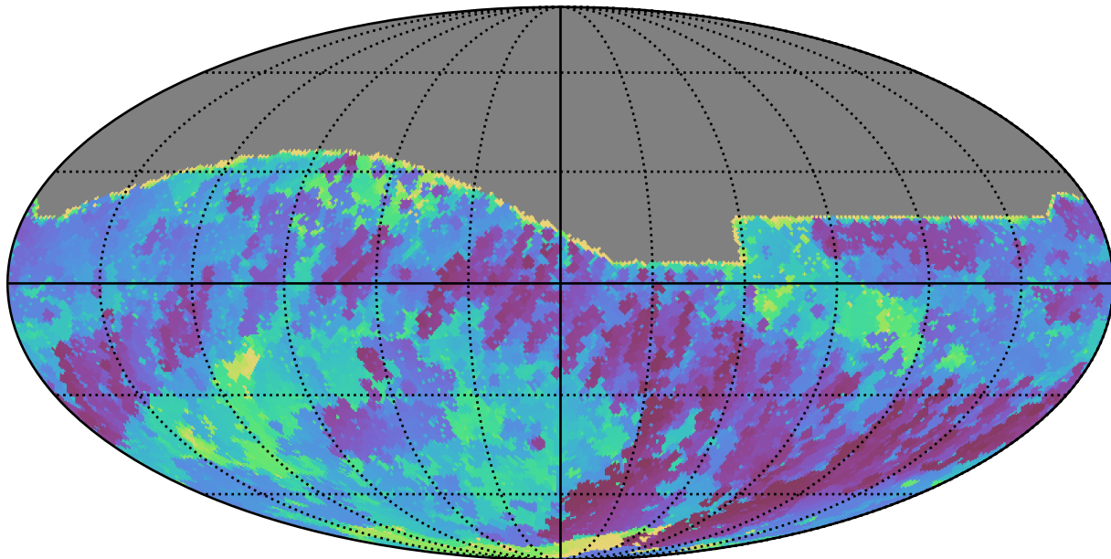
extra_ss_neo3_v3.4_10yrs All sky r band: Min skyBrightness
