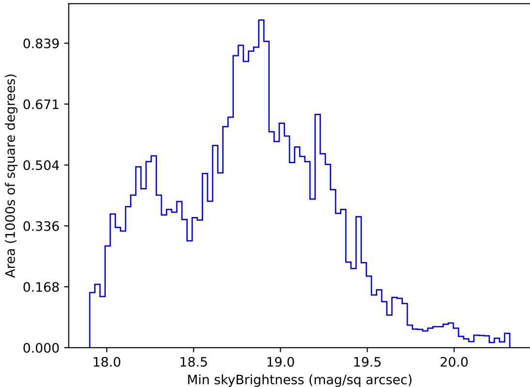
extra_ss_neo3_v3.4_10yrs All sky r band: Min skyBrightness
