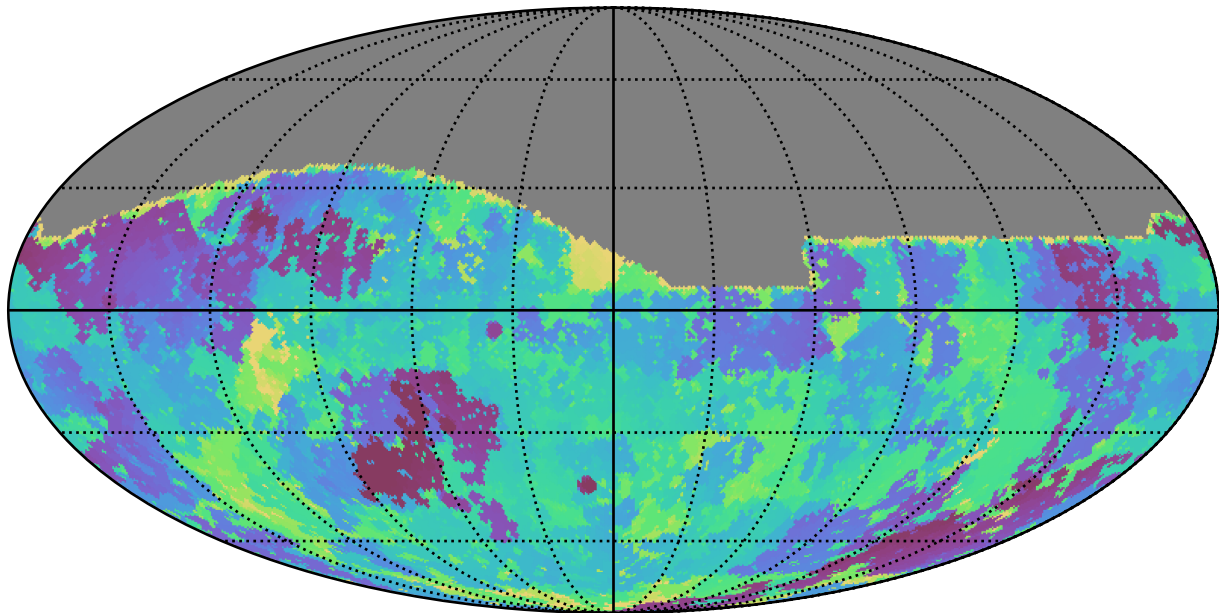
extra_ss_neo3_v3.4_10yrs All sky g band: Min skyBrightness
