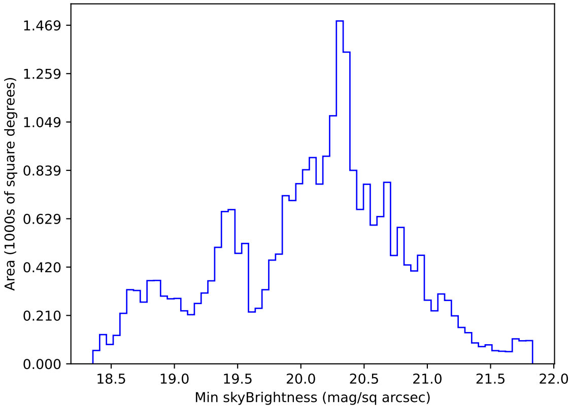
extra_ss_neo3_v3.4_10yrs All sky g band: Min skyBrightness
