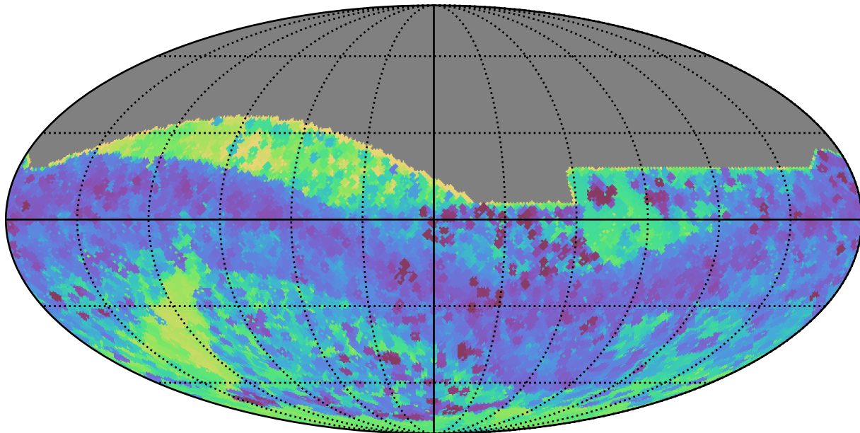
extra_ss_neo3_v3.4_10yrs All sky all bands: Min skyBrightness
