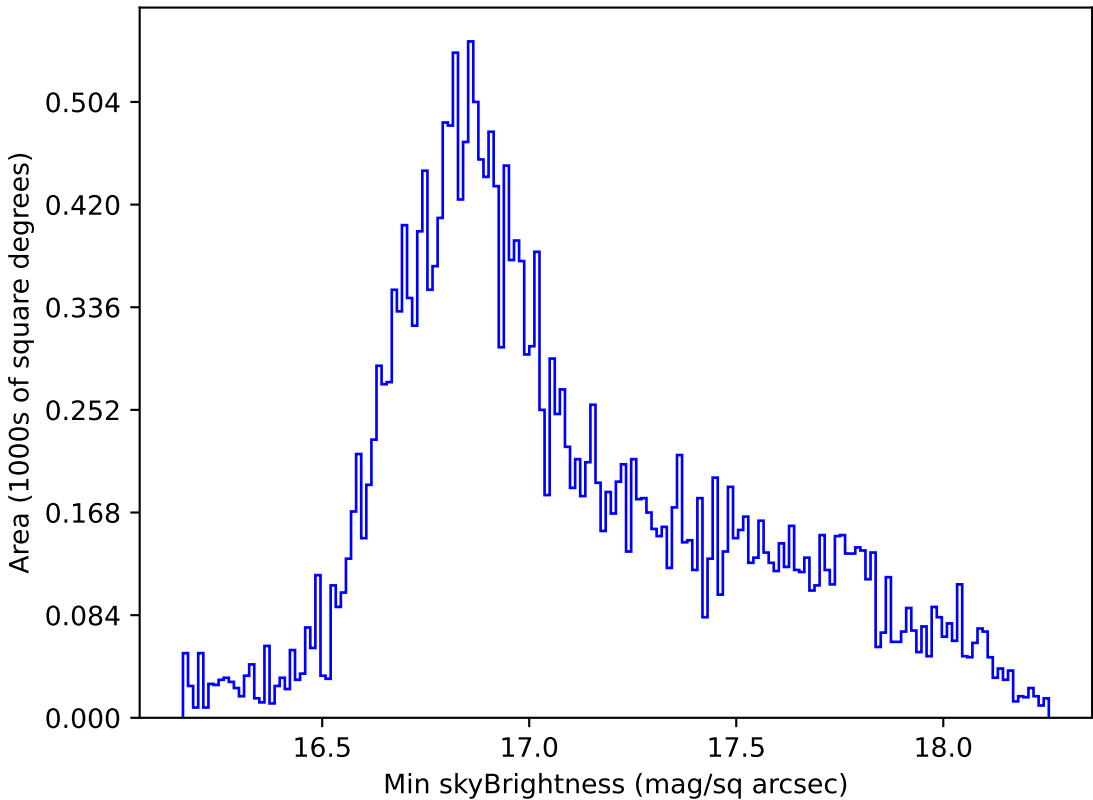
extra_ss_neo3_v3.4_10yrs All sky all bands: Min skyBrightness
