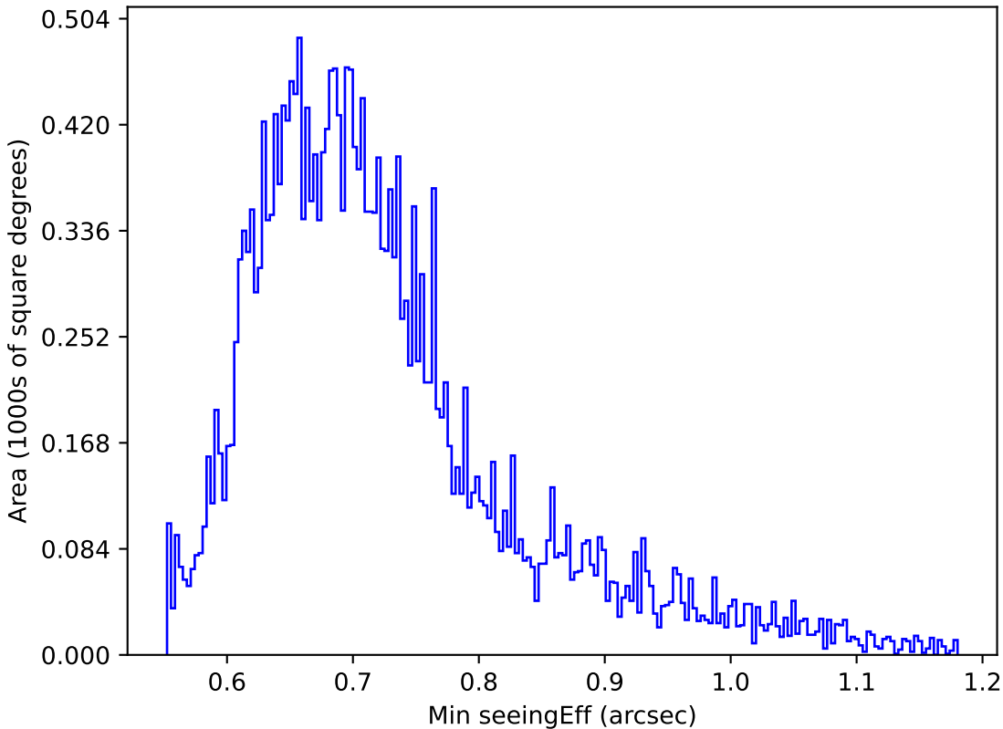
extra_ss_neo3_v3.4_10yrs Yr 1 z band: Min seeingEff
