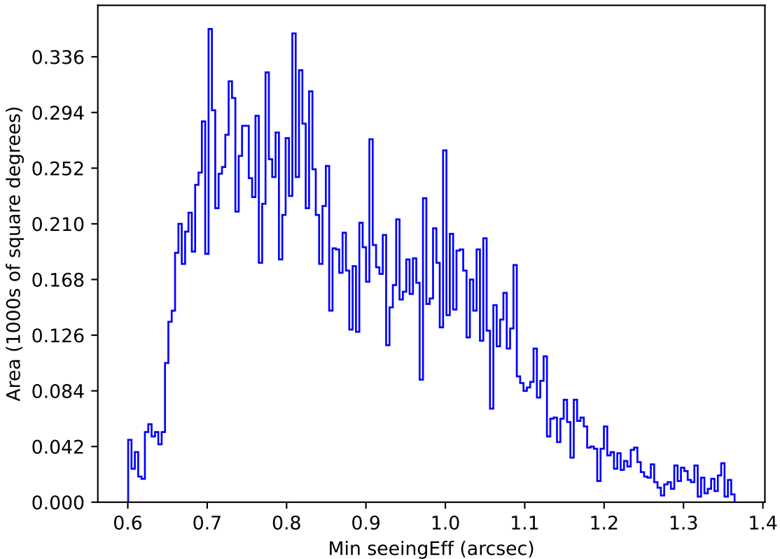
extra_ss_neo3_v3.4_10yrs Yr 1 u band: Min seeingEff
