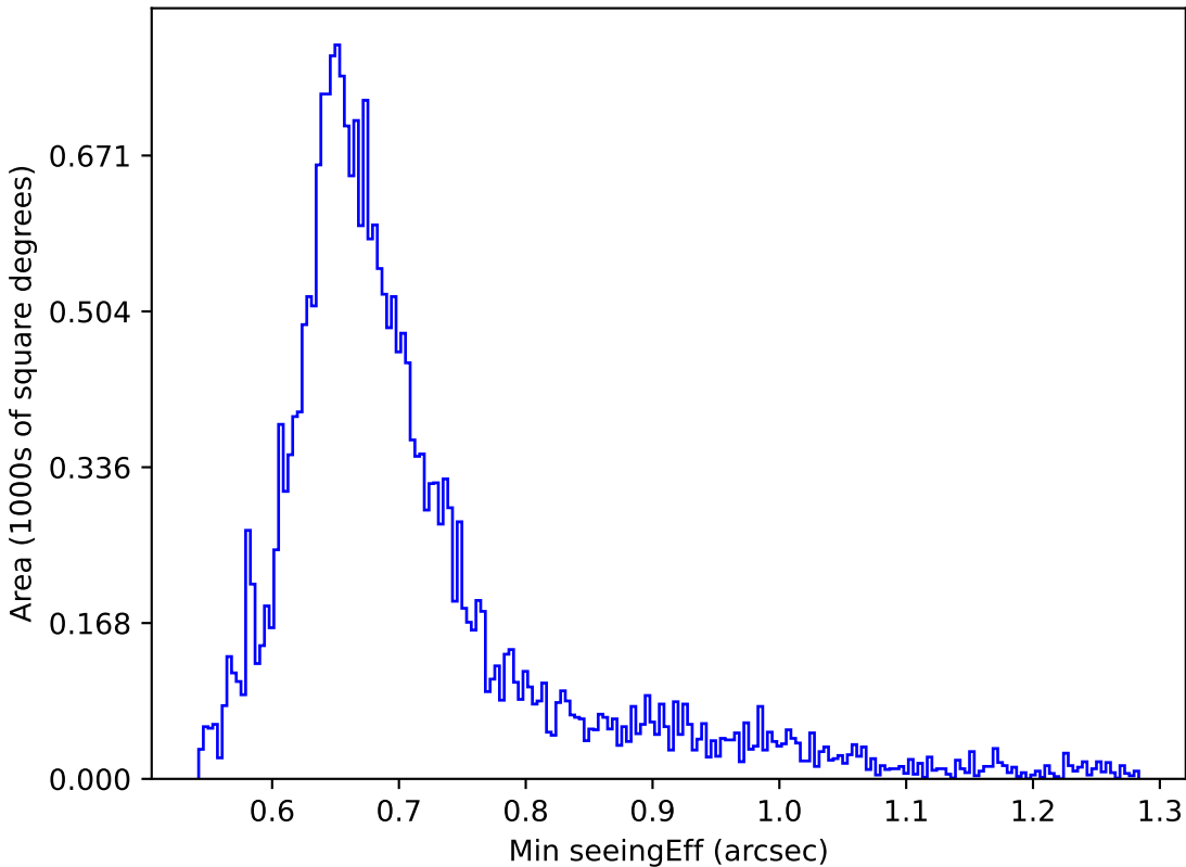
extra_ss_neo3_v3.4_10yrs Yr 1 i band: Min seeingEff
