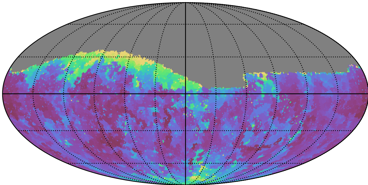
extra_ss_neo3_v3.4_10yrs Yr 1 g band: Min seeingEff
