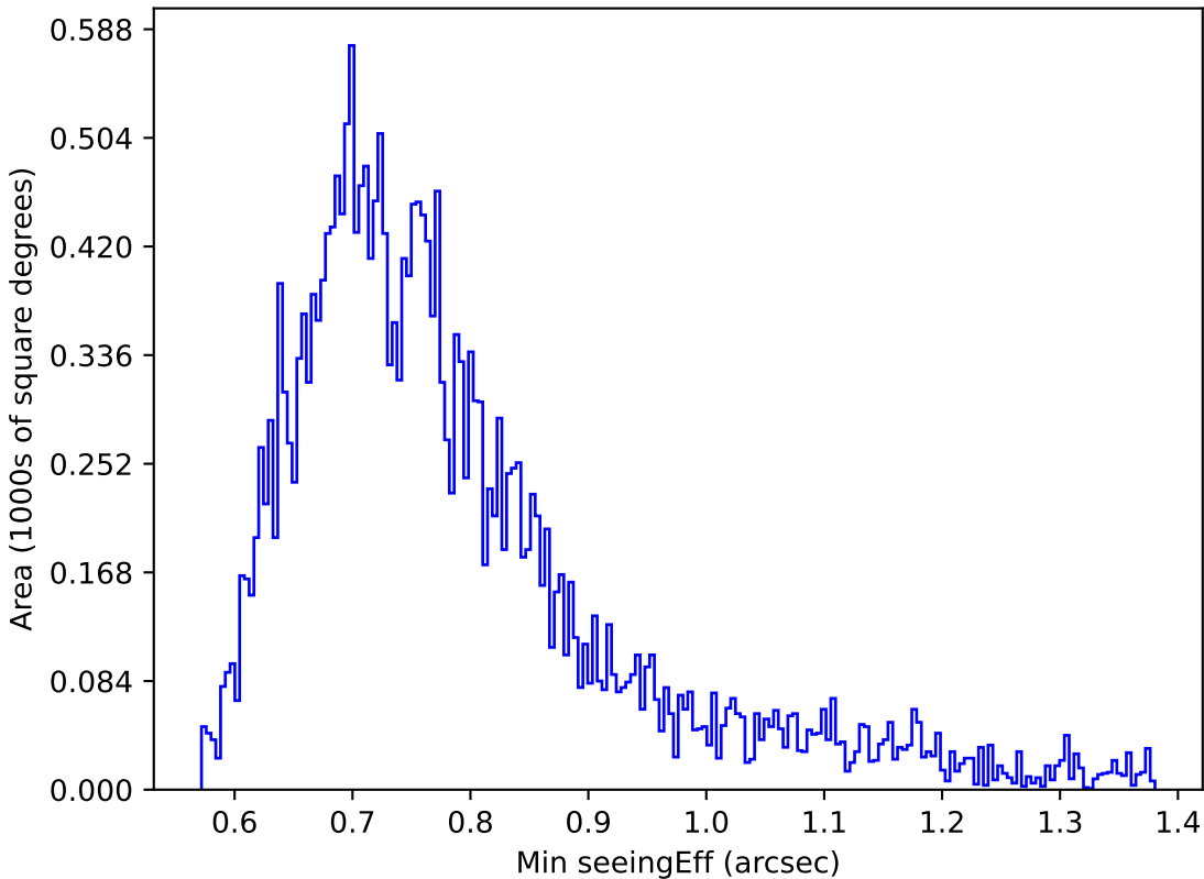
extra_ss_neo3_v3.4_10yrs Yr 1 g band: Min seeingEff
