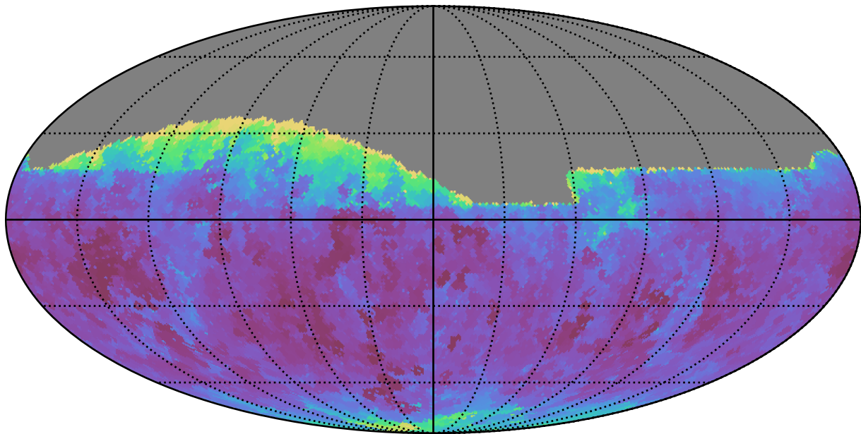
extra_ss_neo3_v3.4_10yrs Yr 1 all bands: Min seeingEff
