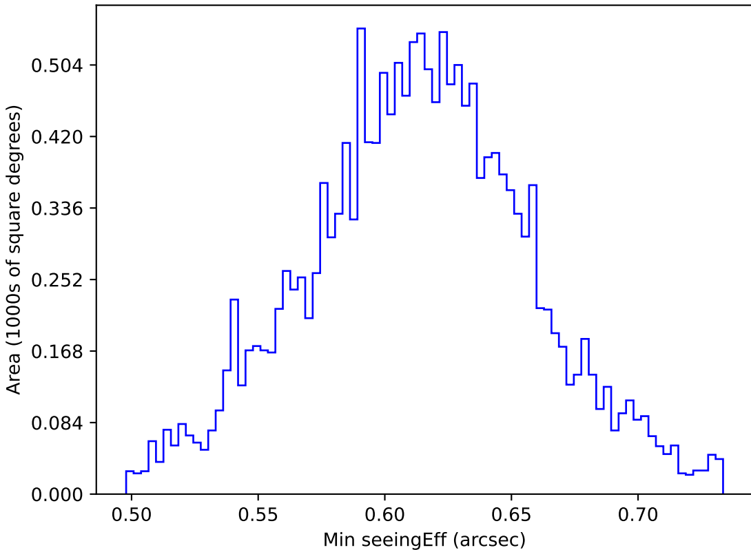
extra_ss_neo3_v3.4_10yrs WFD r band: Min seeingEff
