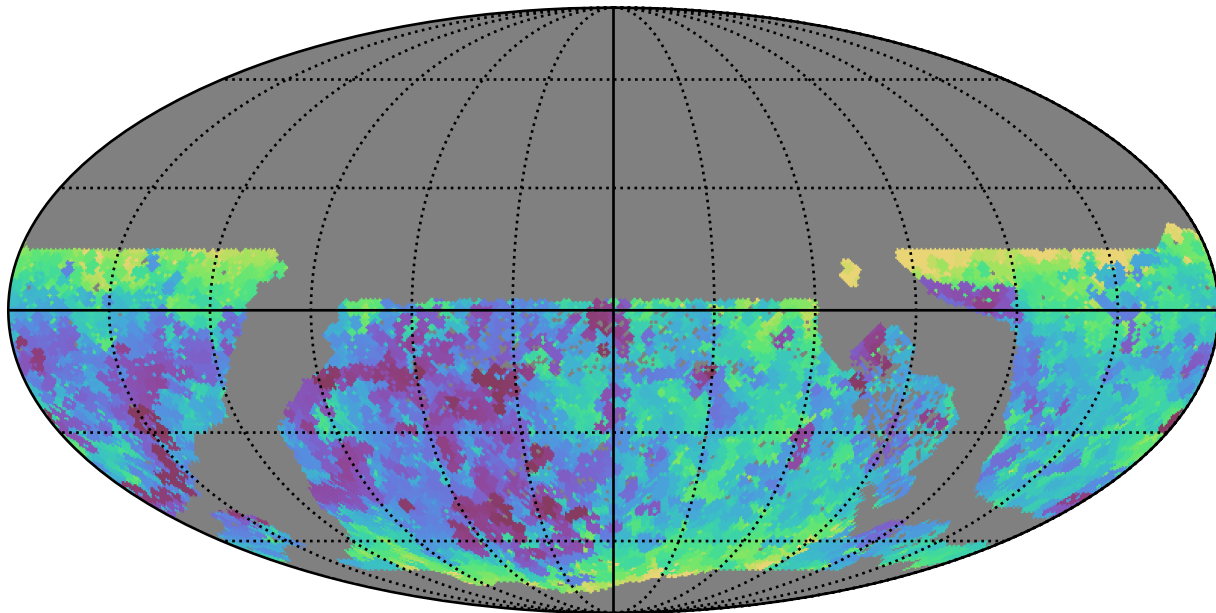
extra_ss_neo3_v3.4_10yrs WFD i band: Min seeingEff
