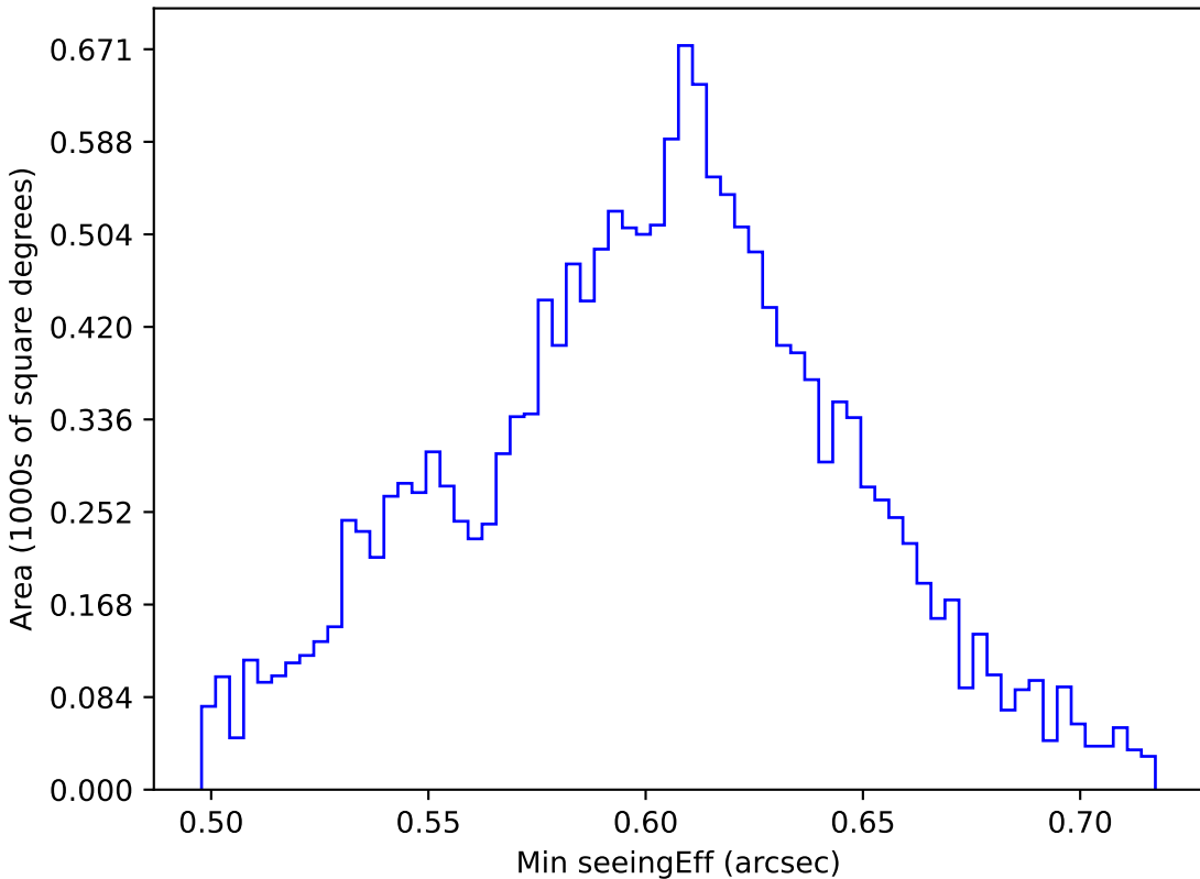
extra_ss_neo3_v3.4_10yrs WFD i band: Min seeingEff
