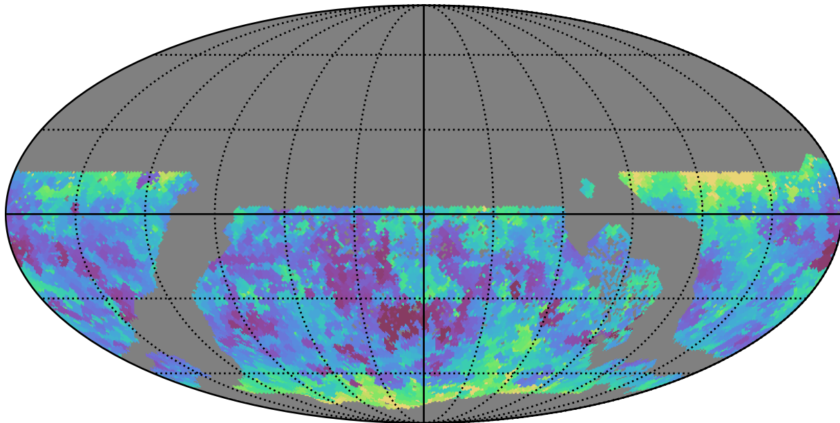
extra_ss_neo3_v3.4_10yrs WFD g band: Min seeingEff
