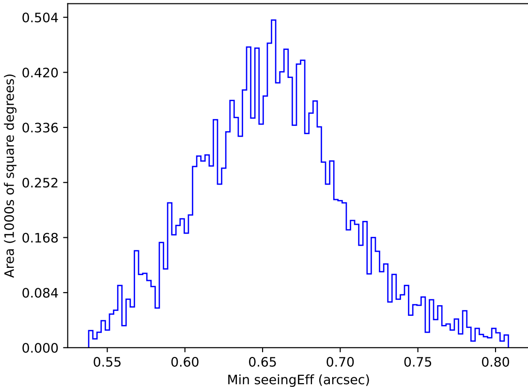
extra_ss_neo3_v3.4_10yrs WFD g band: Min seeingEff
