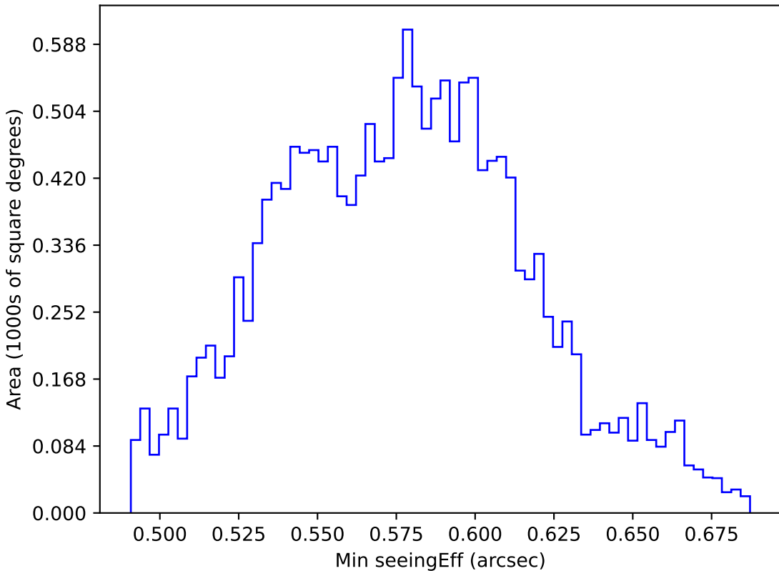
extra_ss_neo3_v3.4_10yrs WFD all bands: Min seeingEff
