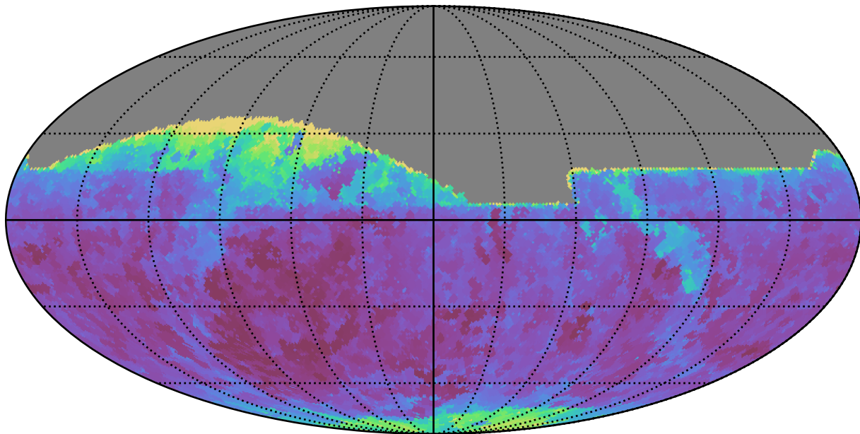
extra_ss_neo3_v3.4_10yrs All sky z band: Min seeingEff
