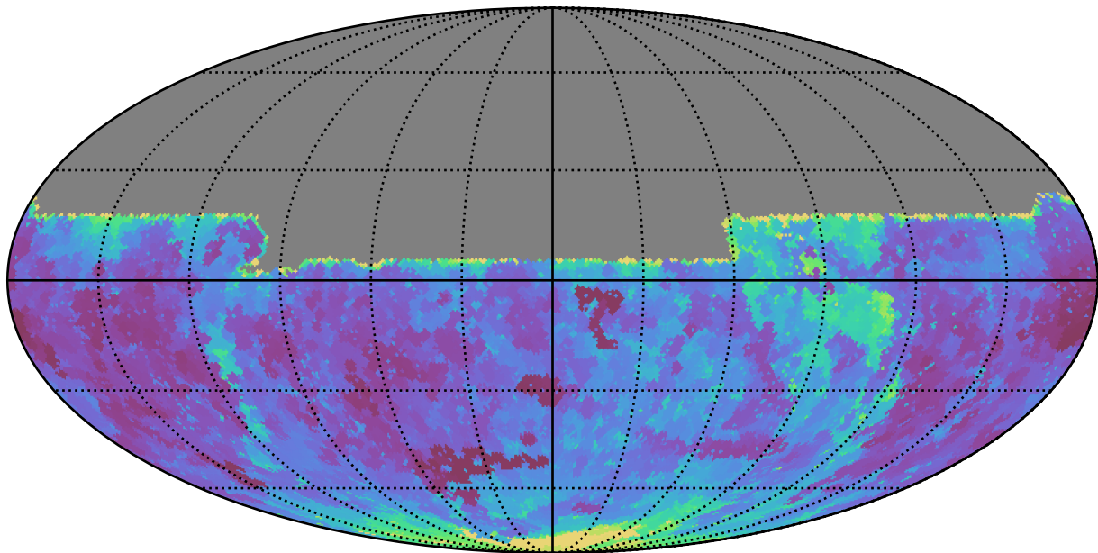
extra_ss_neo3_v3.4_10yrs All sky u band: Min seeingEff
