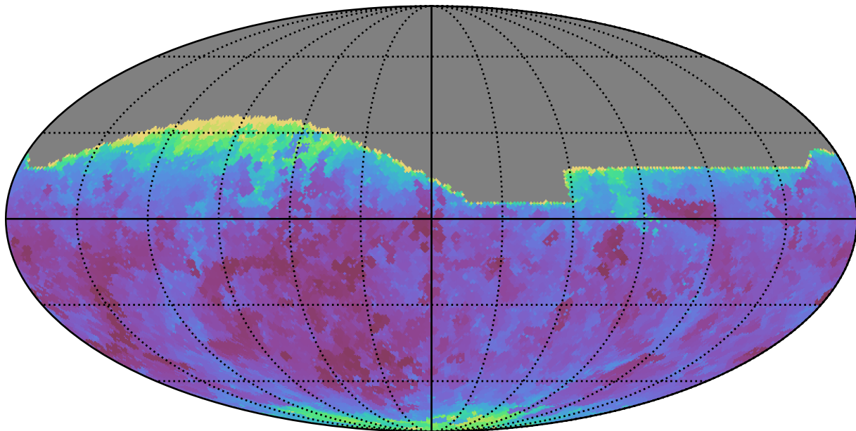
extra_ss_neo3_v3.4_10yrs All sky i band: Min seeingEff
