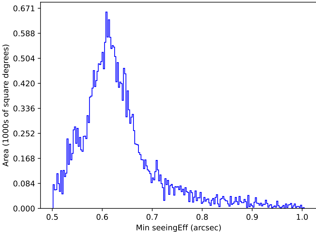
extra_ss_neo3_v3.4_10yrs All sky i band: Min seeingEff
