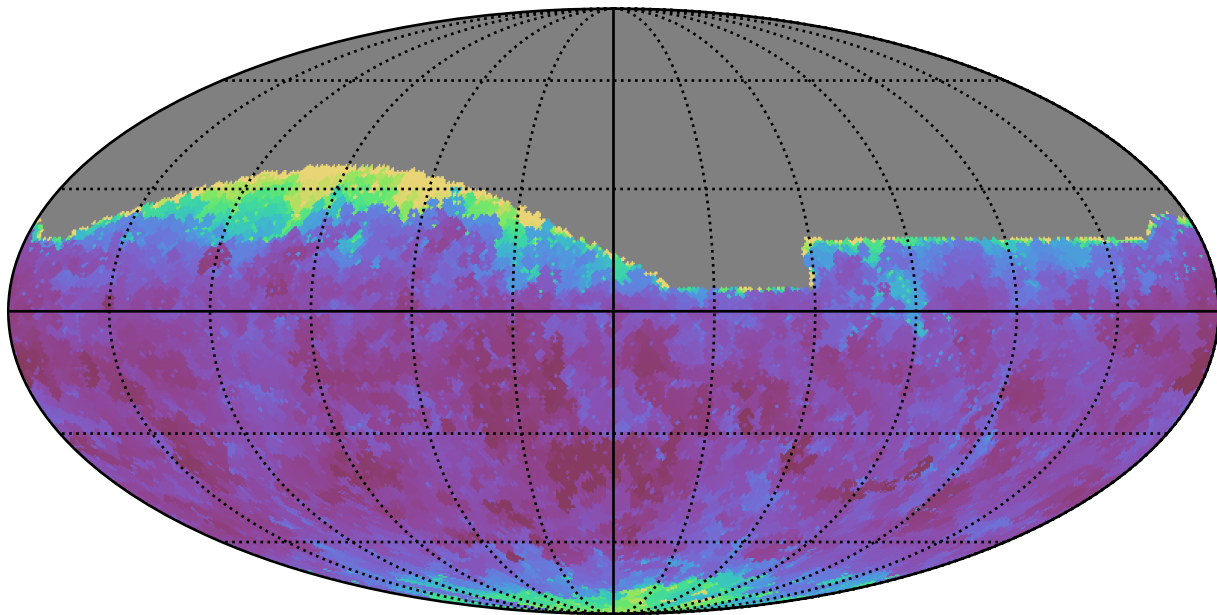
extra_ss_neo3_v3.4_10yrs All sky g band: Min seeingEff
