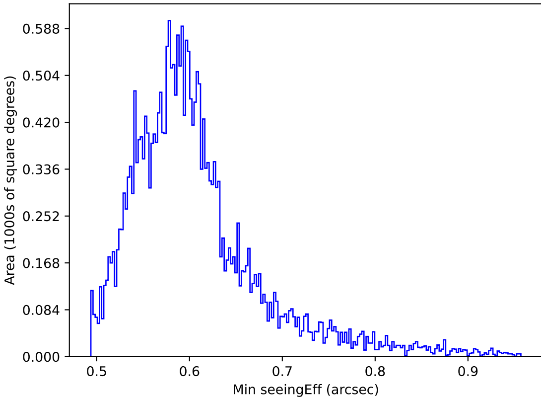
extra_ss_neo3_v3.4_10yrs All sky all bands: Min seeingEff
