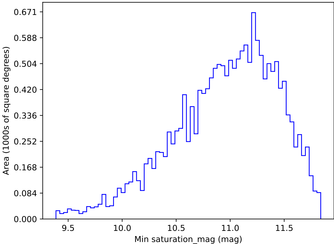
extra_ss_neo3_v3.4_10yrs WFD all bands: Min saturation_mag
