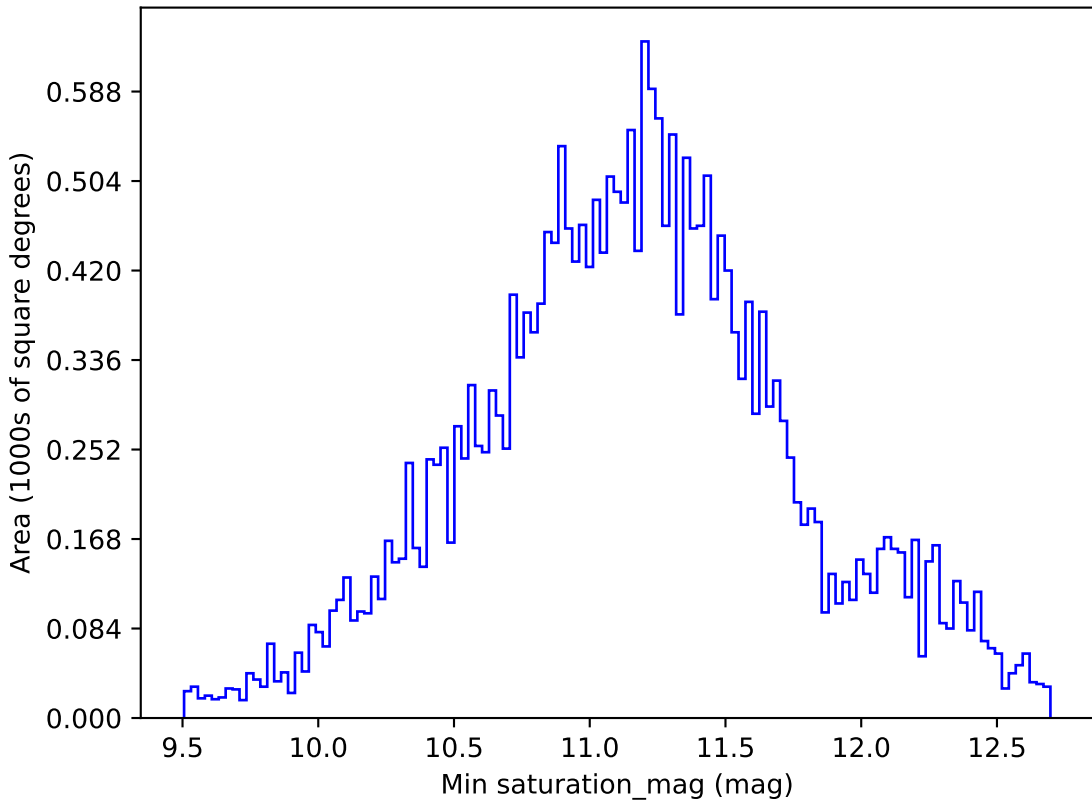
extra_ss_neo3_v3.4_10yrs All sky all bands: Min saturation_mag
