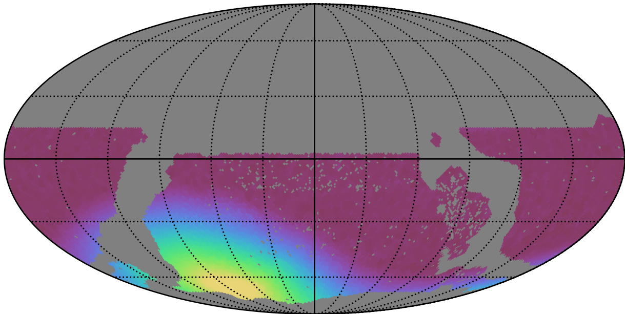
extra_ss_neo3_v3.4_10yrs WFD all bands: Min moonDistance
