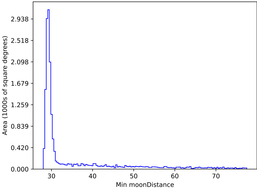
extra_ss_neo3_v3.4_10yrs WFD all bands: Min moonDistance
