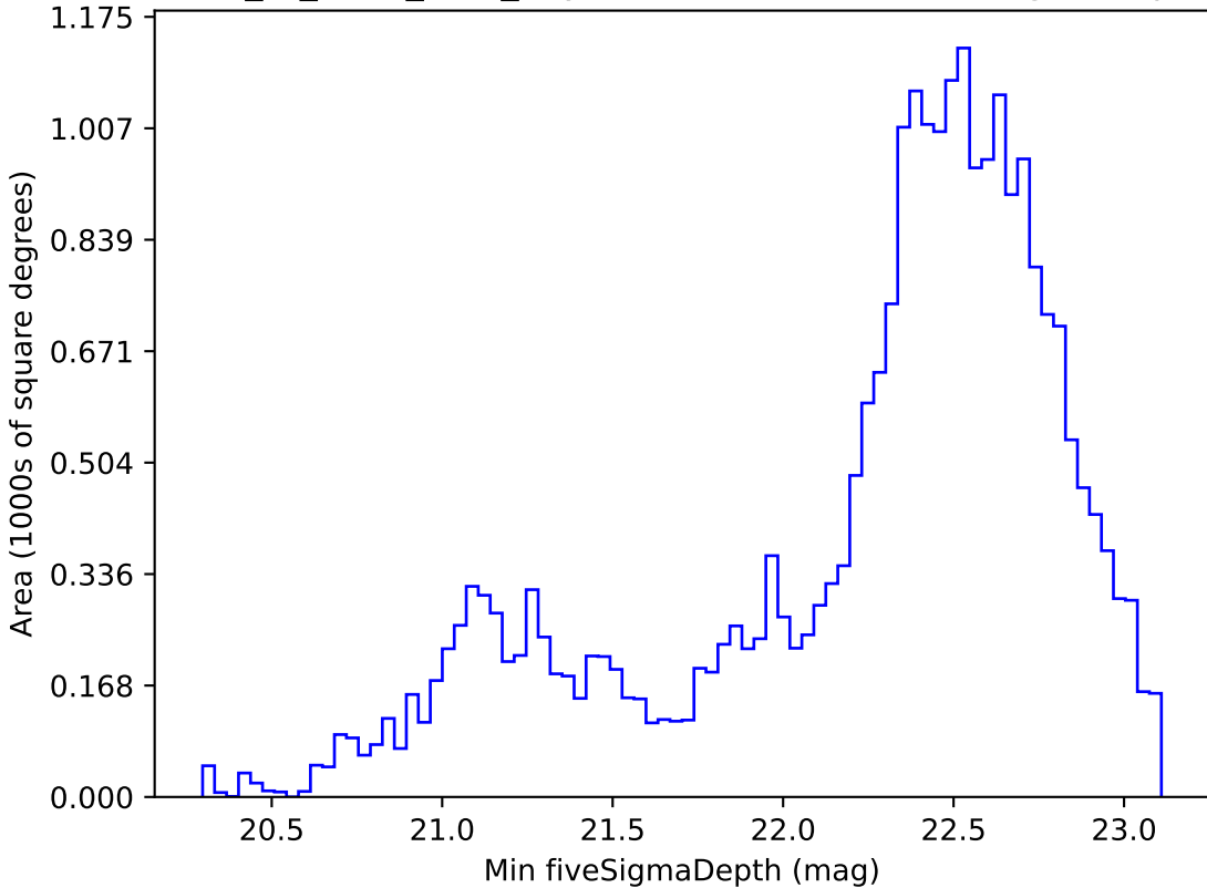
extra_ss_neo3_v3.4_10yrs Yr 1 z band: Min fiveSigmaDepth
