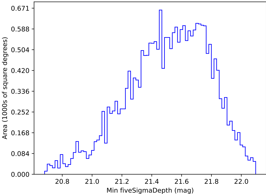
extra_ss_neo3_v3.4_10yrs Yr 1 y band: Min fiveSigmaDepth
