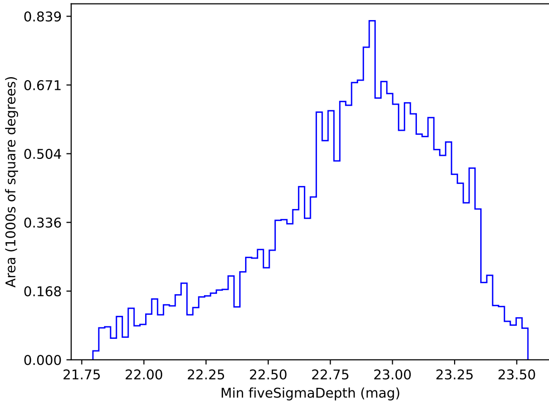
extra_ss_neo3_v3.4_10yrs Yr 1 u band: Min fiveSigmaDepth
