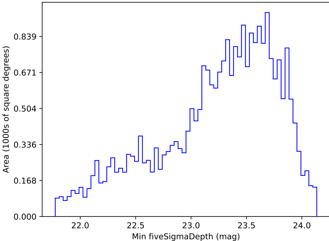
extra_ss_neo3_v3.4_10yrs Yr 1 r band: Min fiveSigmaDepth
