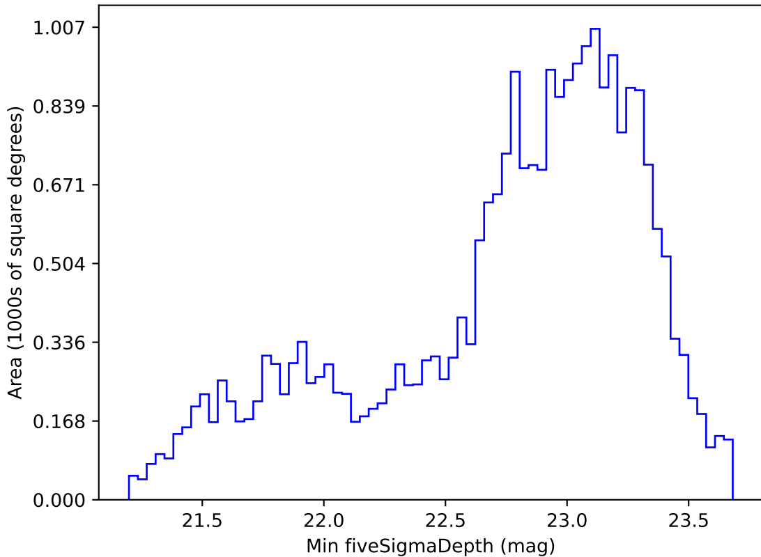
extra_ss_neo3_v3.4_10yrs Yr 1 i band: Min fiveSigmaDepth
