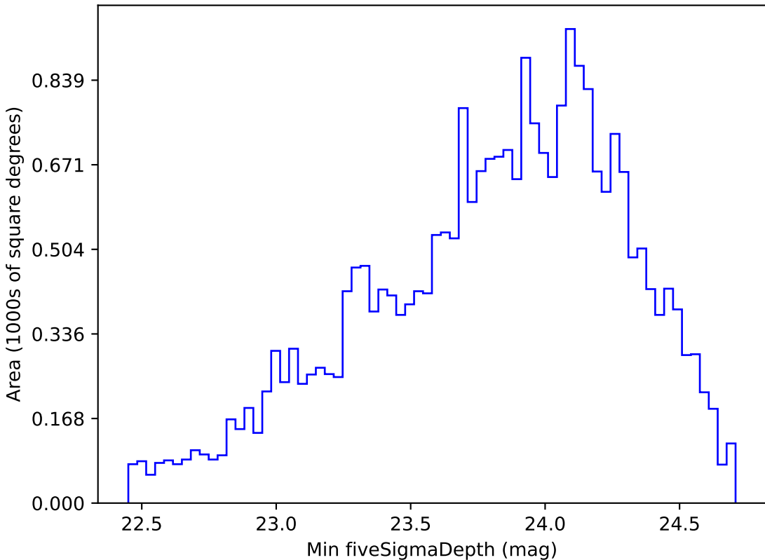
extra_ss_neo3_v3.4_10yrs Yr 1 g band: Min fiveSigmaDepth
