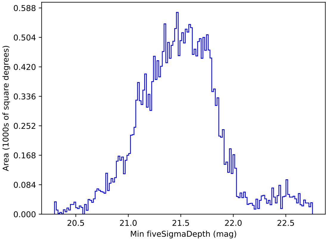
extra_ss_neo3_v3.4_10yrs Yr 1 all bands: Min fiveSigmaDepth
