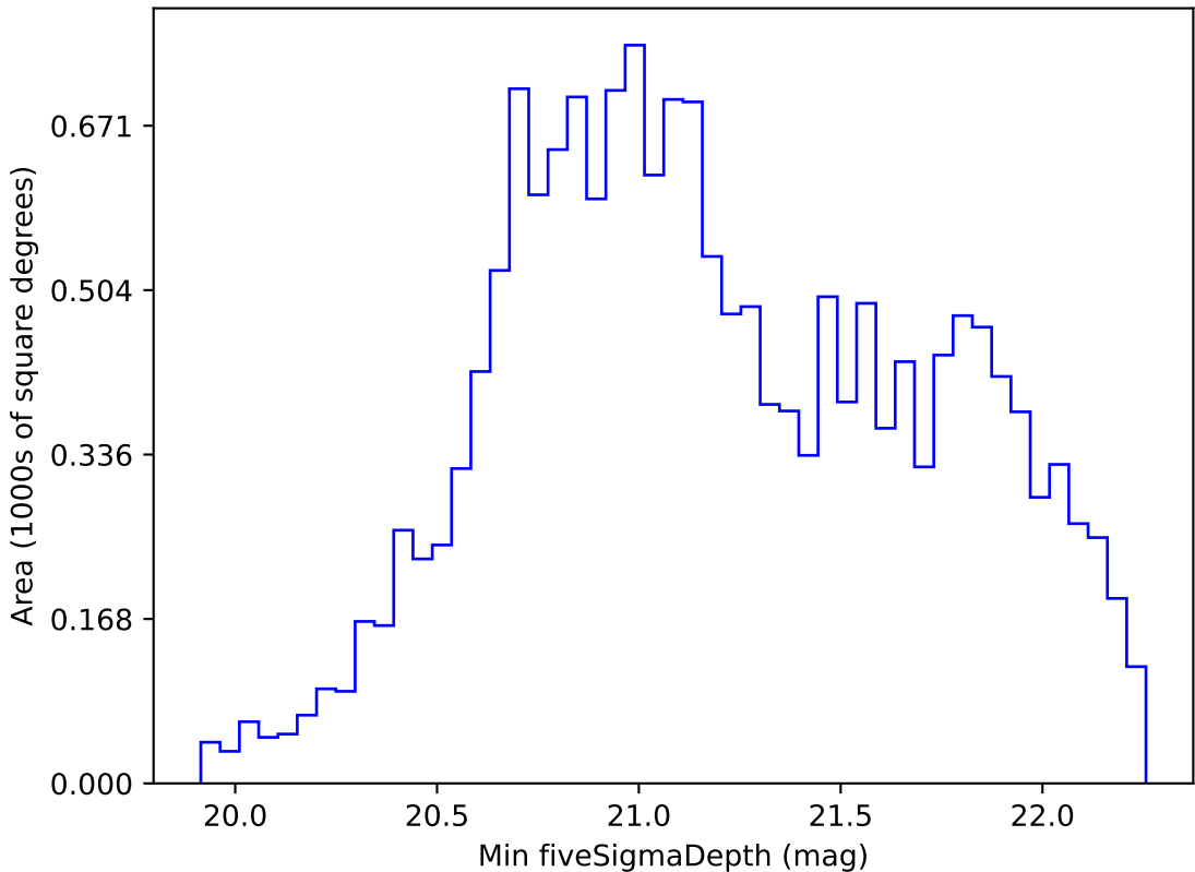
extra_ss_neo3_v3.4_10yrs WFD z band: Min fiveSigmaDepth
