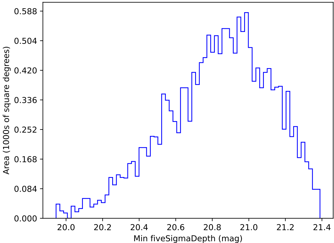
extra_ss_neo3_v3.4_10yrs WFD y band: Min fiveSigmaDepth
