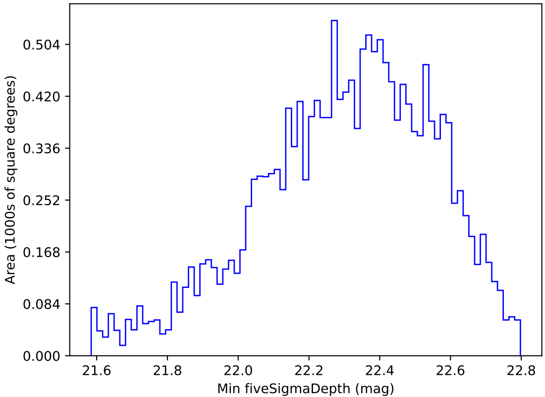
extra_ss_neo3_v3.4_10yrs WFD u band: Min fiveSigmaDepth
