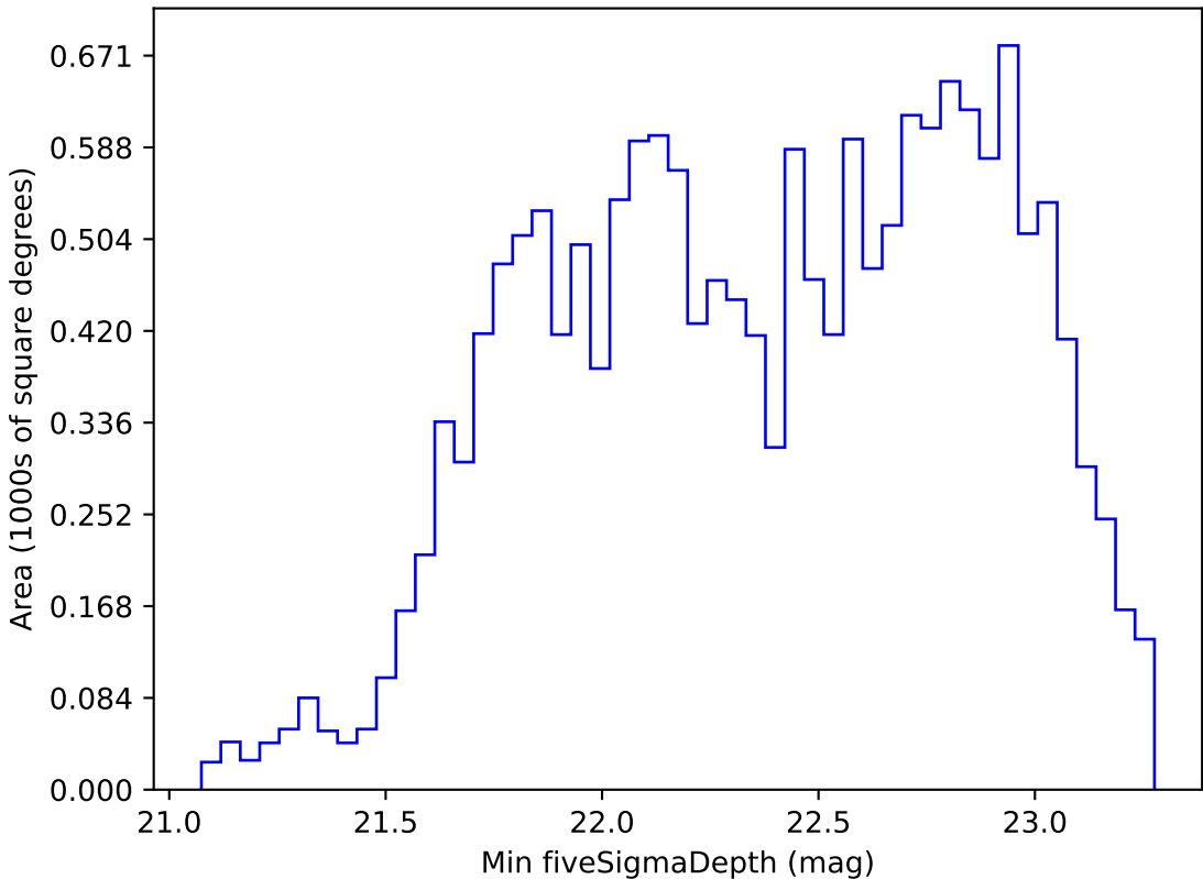
extra_ss_neo3_v3.4_10yrs WFD r band: Min fiveSigmaDepth
